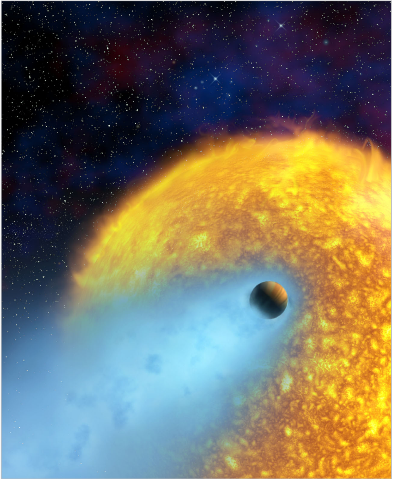
This artist's impression shows a dramatic close-up of the scorched extrasolar planet HD 209458b in its orbit 'only' 7 million kilometres from its yellow Sun-like star. The planet is a type of extrasolar planet known as a 'hot Jupiter'.
