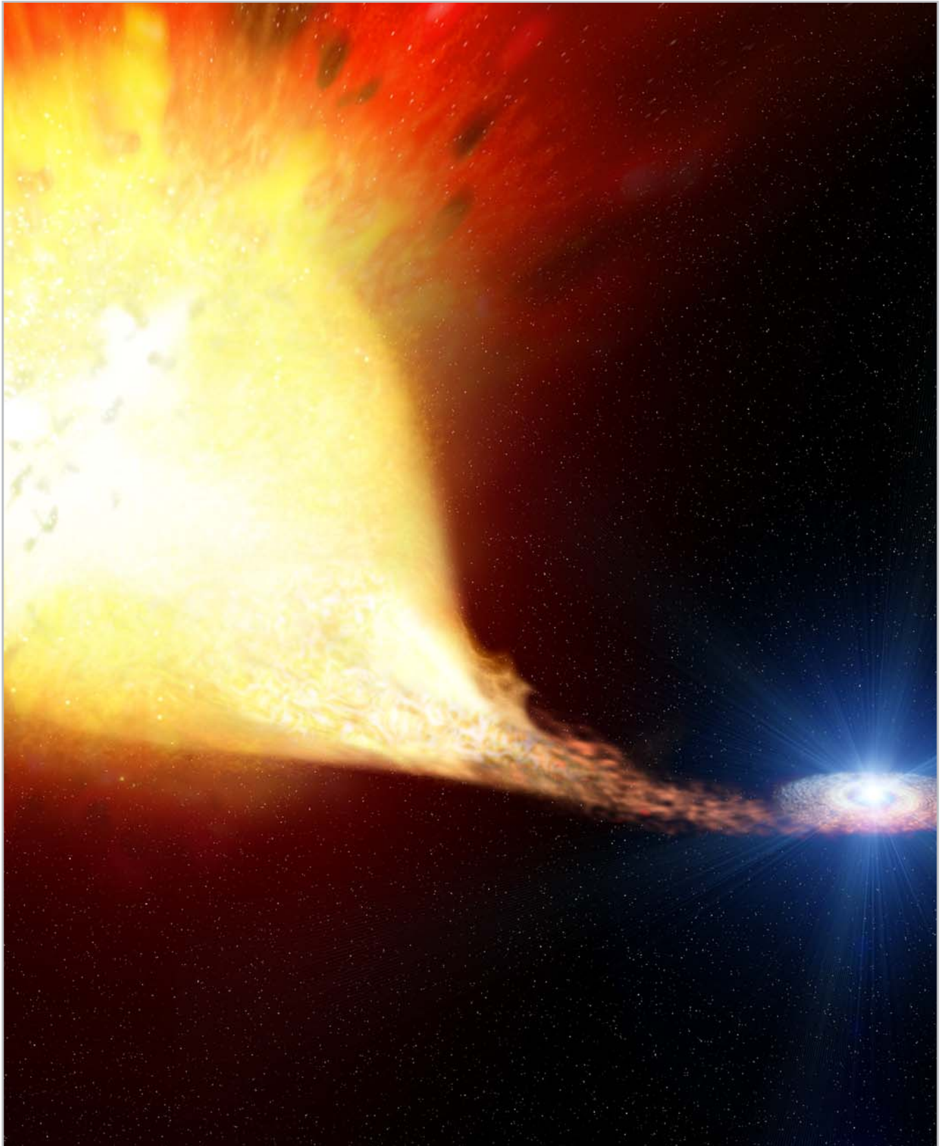
(Artist's impression) A joint European/University of Hawaii team of astronomers has for the first time observed a stellar survivor to emerge from a double star system involving an exploded supernova.
