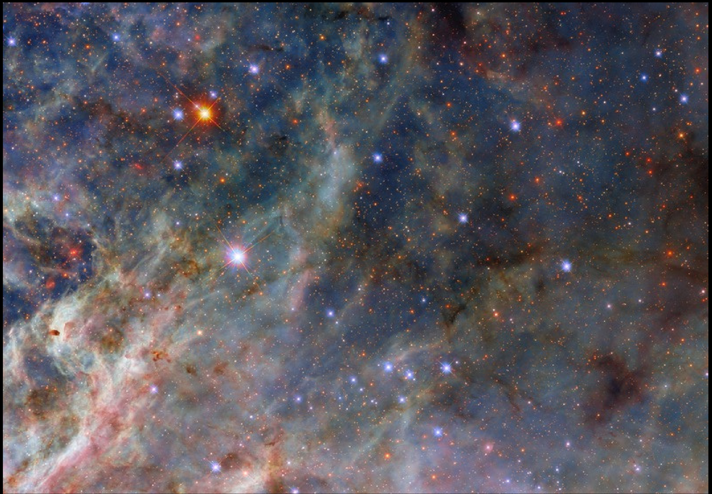
Tarantula Nebula
